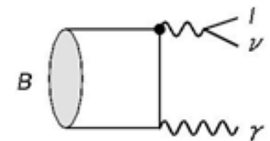
Fig.2 : radiative decay of B meson
