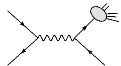
Fig.1: meson production in e^+e^- collision
